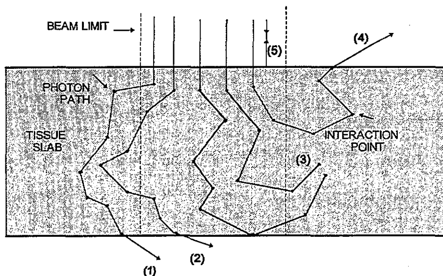
Figure 1. Types of photon path passing through a tissue slab. The paths considered in the Monte Carlo code are the following: diffuse transmittance T (1 + 2); collimated transmittance T_c (2); fraction absorbed A (3); diffuse reflectance \gamma (4); specular (Fresnel) reflectance f (5); total reflectance R (4 + 5).
